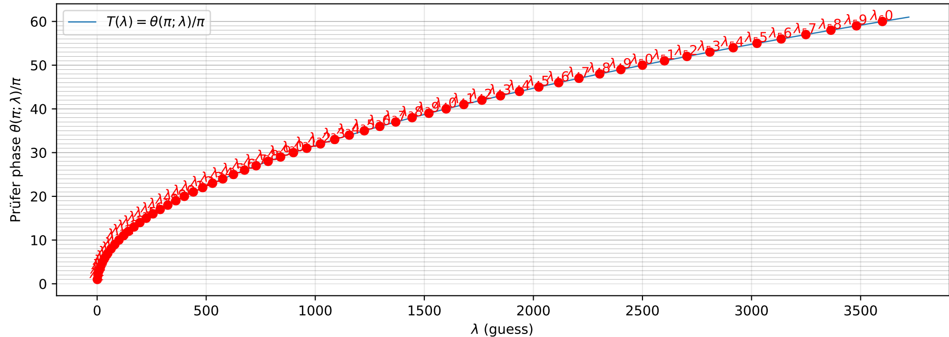
Prüfer phase sweep on graded grid (n=100, ratio=1.3) for 60 eigenvalues
